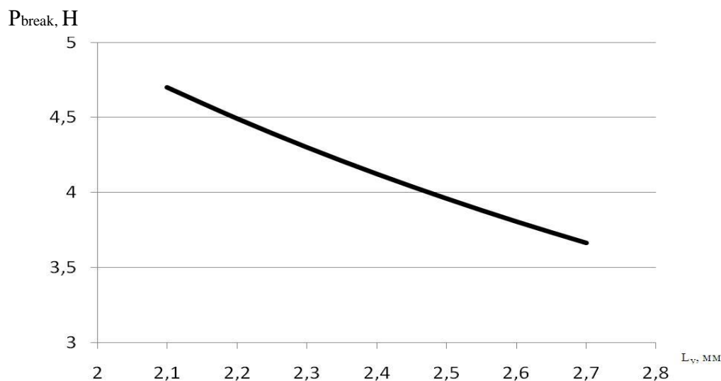
Figure 2 – The dependence of the disruptive pressure value p_{break} on the geometric density on the weft L_y of the woven reinforcing frame of the latex PFH with a diameter of 77 mm
