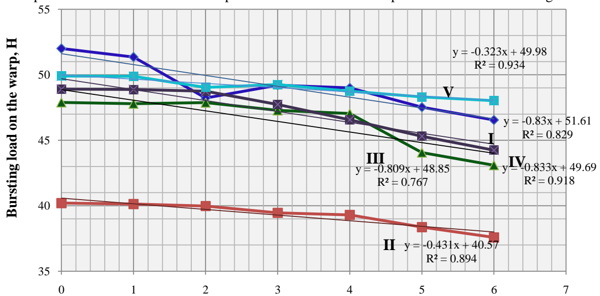
Figure 1 – Indicators of bursting load changes of the fabric on the warp
