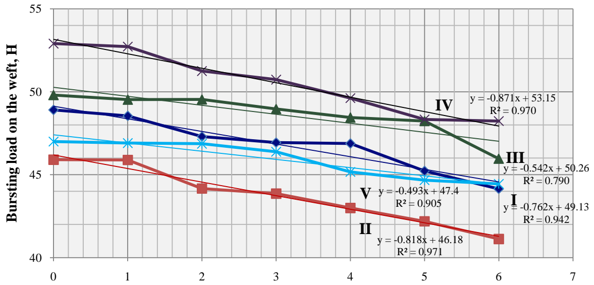
Figure 2 - Indicators of bursting load changes of the fabric on the weft
